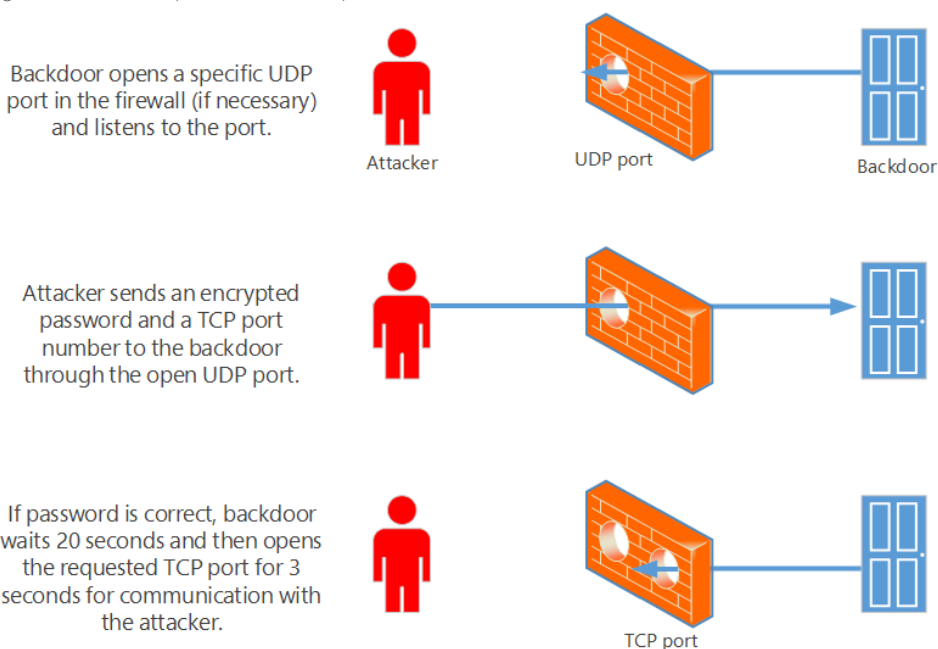
Figure 14. How the Dipsind knocker component communicates with an attacker
