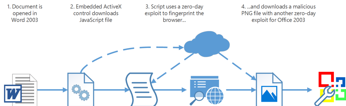
Figure 8. An exploit mechanism used by PLATINUM
