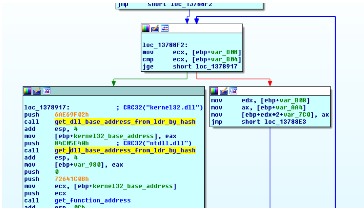
A snippet of shellcode 3's code as viewed in IDA Pro.
