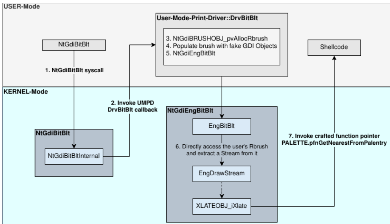
Figure 17: Control flow of the EpMe exploit of CVE-2017-0005.
