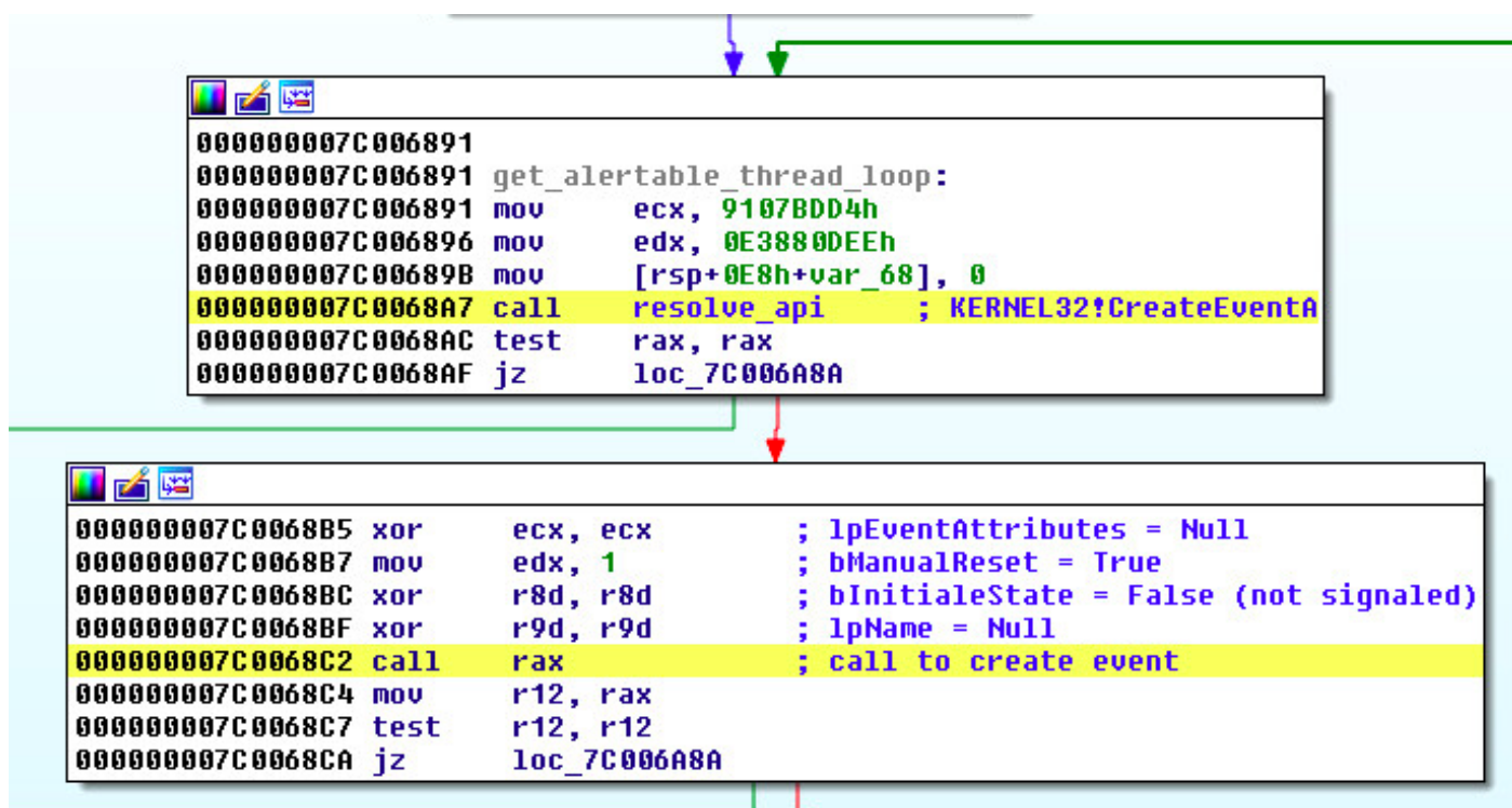
Figure 2: The call to kernel32!CreateEventA.
