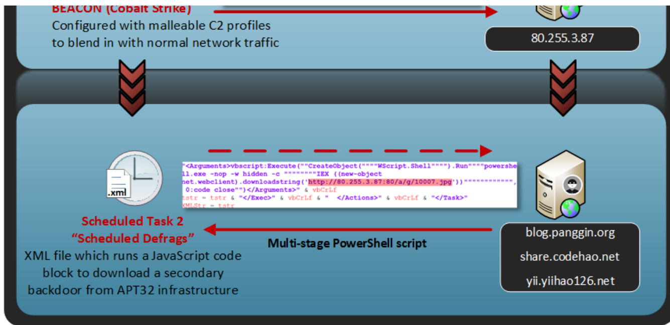
Figure 5: APT32 Phishing Chain of Events
