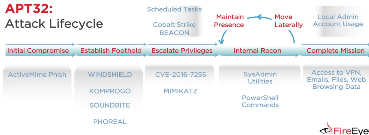
Figure 6: APT32 Attack Lifecycle
