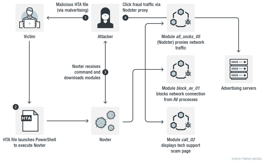
Figure 1. Infection chain of KovCoreG, Novter, and Nodster
