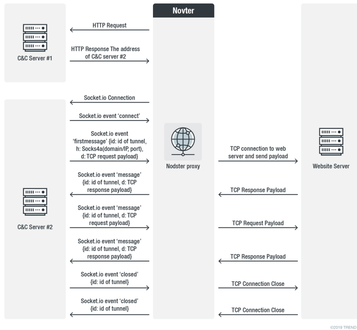
Figure 4. The communication flow between the Nodster proxy and C&C servers
