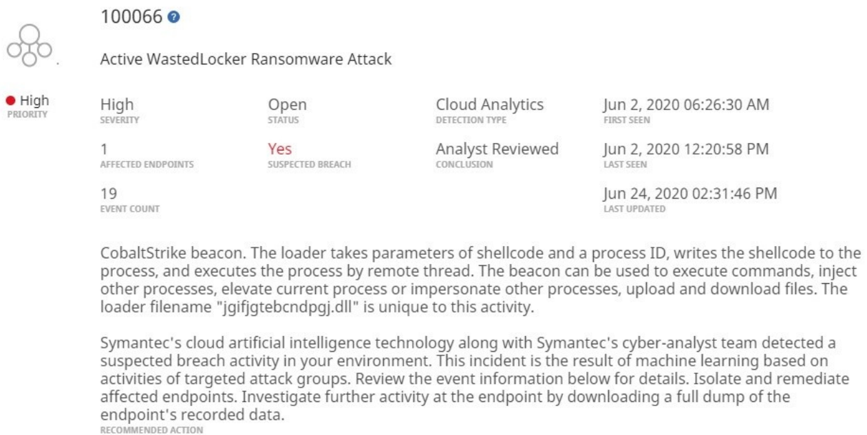
Figure 1. Example of Targeted Attack Cloud Analytics alert received by Symantec Endpoint Detection and Response (EDR) customers, warning them of early stage WastedLocker activity on their networks
