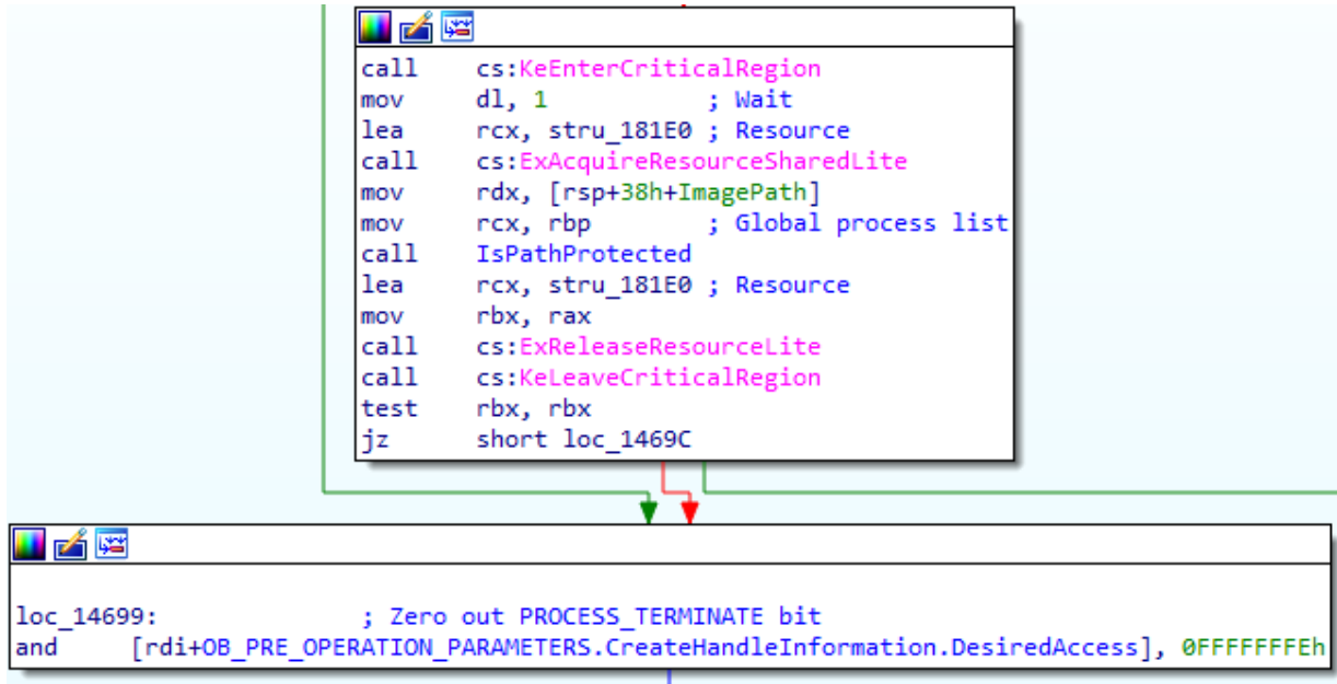
Figure 10: Unsetting the PROCESS_TERMINATE bit of DesiredAccess
