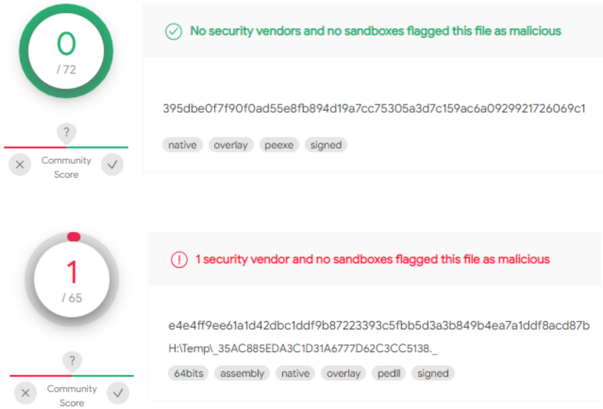
Figure 9: Detection rates of the rootkit samples from VirusTotal
