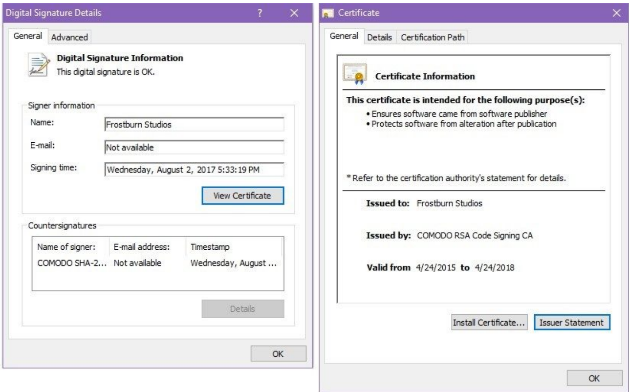
Figure 8: Digital signature of a crtsys.sys driver
