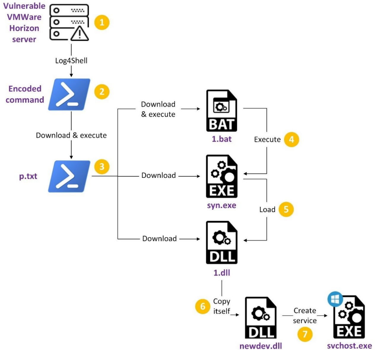
Figure 1: Flow of events from Log4Shell exploitation to execution of the final payload The encoded PowerShell command downloads another PowerShell script from a remote server and executes it.
