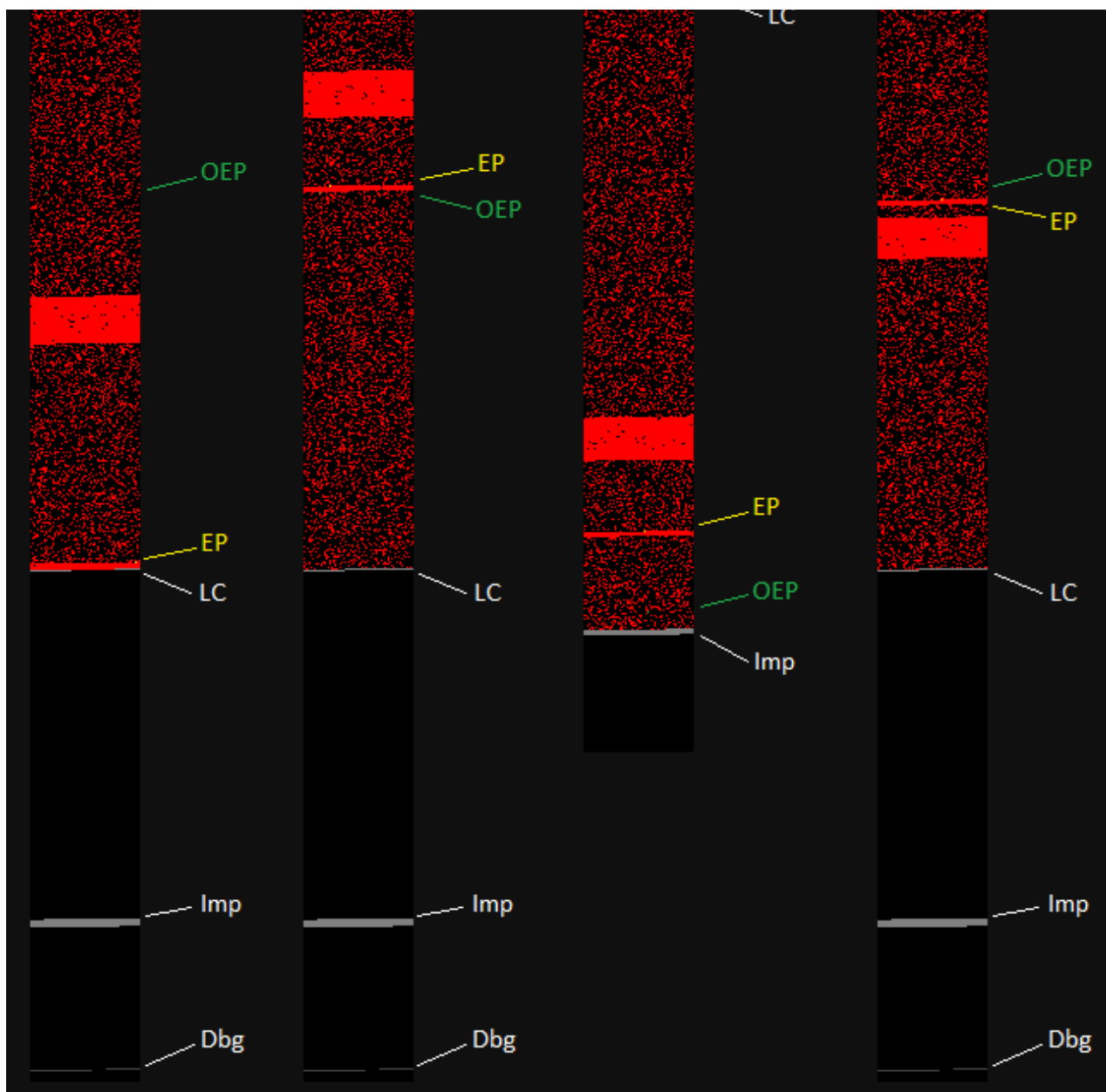
Figure 3. File locations of modifications (red) and the PE structures they avoid (gray). From left to right, the four vertical bars represent the ".text" sections of NOTEPAD2.EXE, Notepad3.exe, Notepad4.exe, and notepad10.exe, as compared to the original Notepad from their respective families. The Import Address Table (IAT), original entry point (OEP, green), malware entry point (EP, yellow), load configuration directory (LC), import directory (Imp), and debug directory (Dbg) are labeled.
