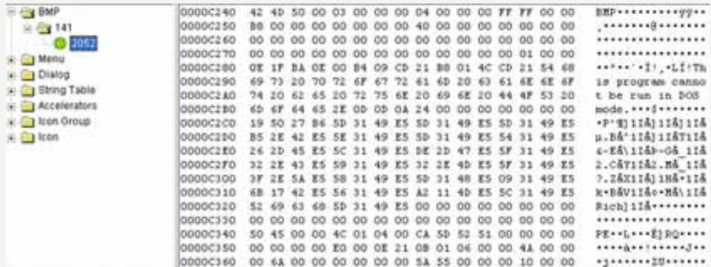
Figure 8: DLL implant embedded in resource section with a fake BMP header
