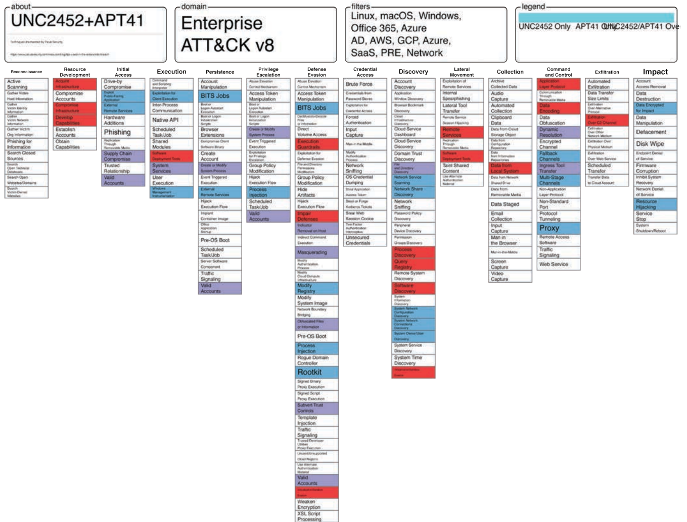
Appendix Figure 3: Visualization of ATT&CK technique comparison between UNC2452 and APT41
