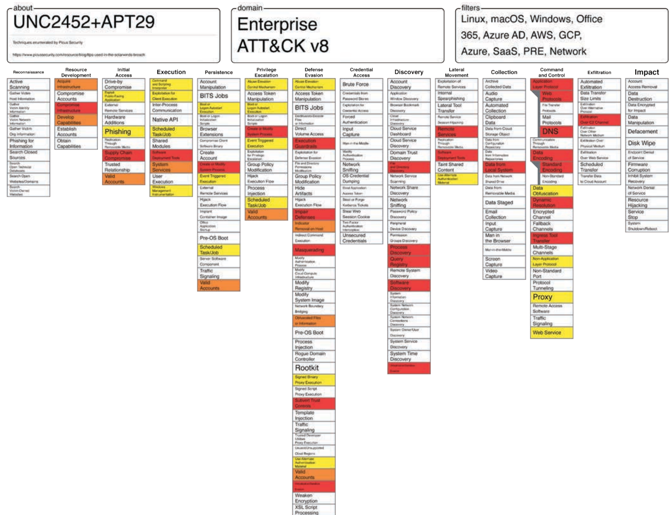
Appendix Figure 2: MITRE ATT&CK mapping of UNC2452 [shown in red] and APT29 [shown in yellow]. Overlapping techniques are shown in orange.
