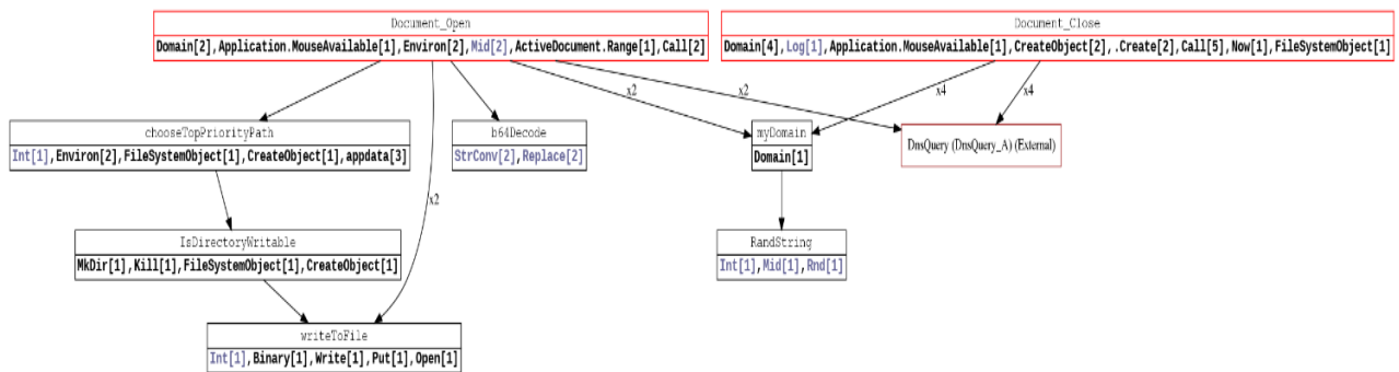
Fig 3: VBA functions call graph generated by Vba2Graph
