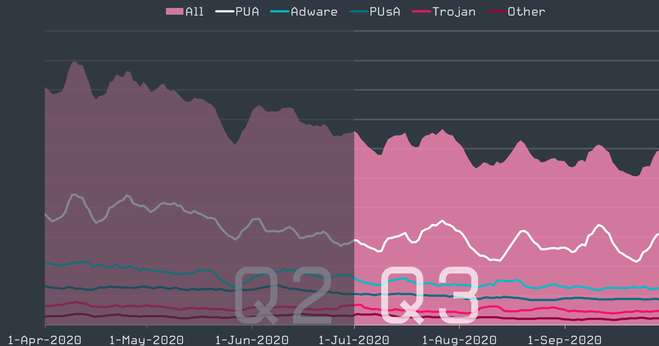
Mac threat detection trend in Q2 2020-Q3 2020, seven-day moving average
