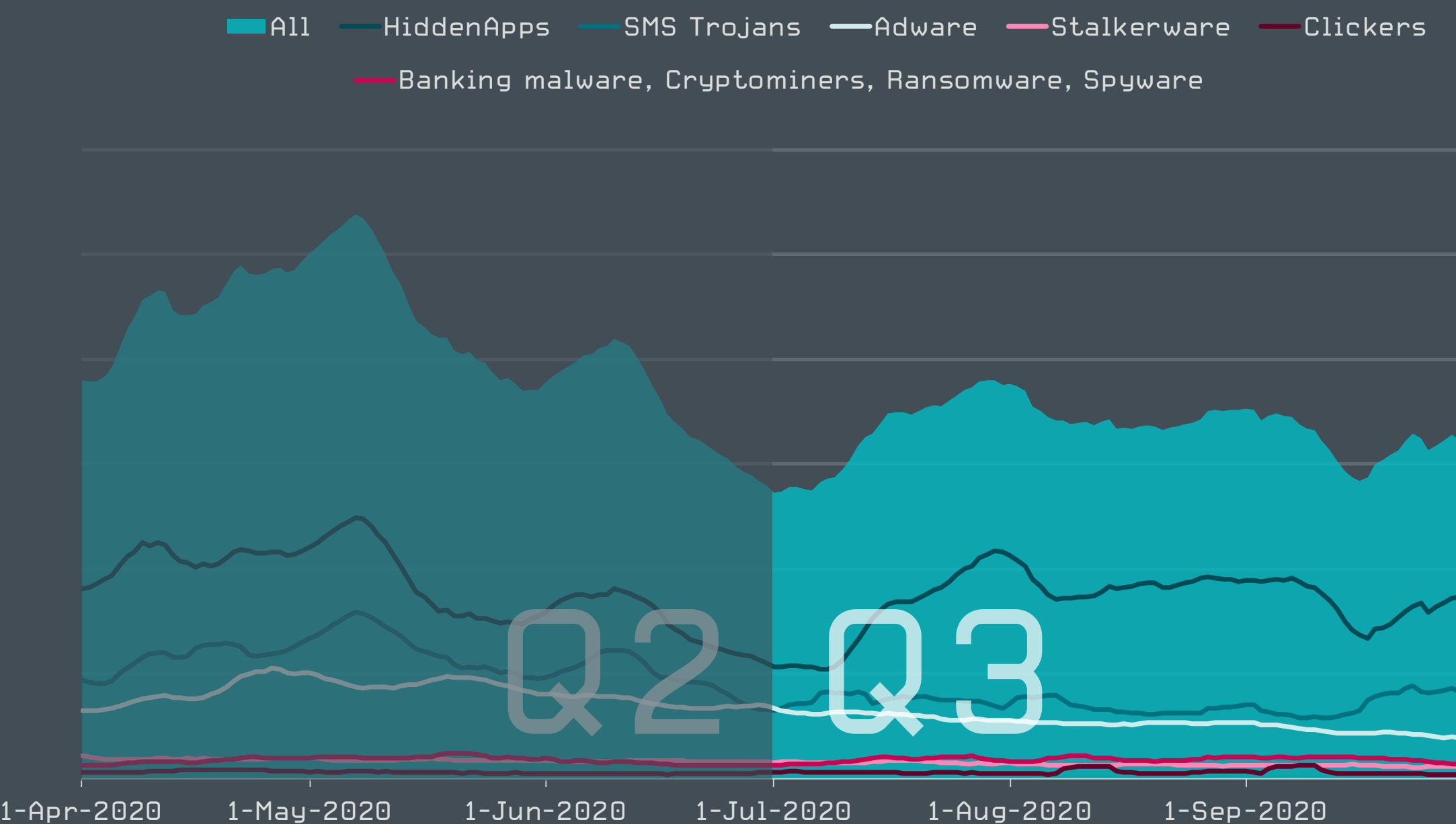
Detection trends of selected Android threat categories in Q2 2020-Q3 2020, seven-day moving average
