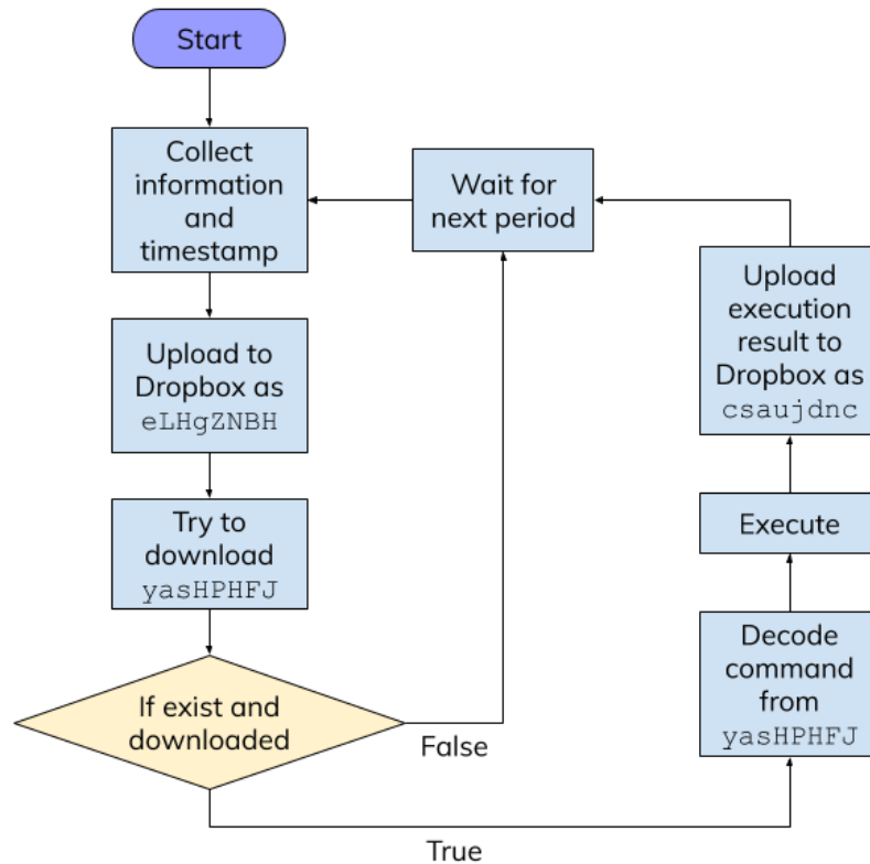
Figure 14. Flow of three files interact with Dropbox
