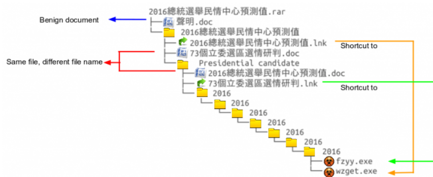
Figure 2: File structure of delivered RAR archive.
