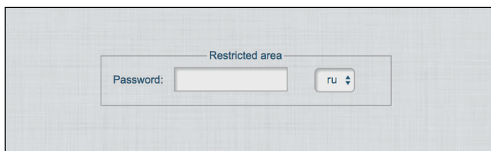
Figure 3: Login page of the C&C server of the Geost botnet. No TLS was used and no username is requested, only a password.
